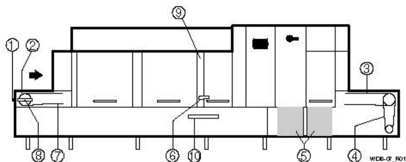
Overview of dishwasher
