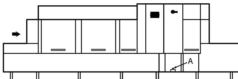
Positioning of earth bolt A = Earth bolt
