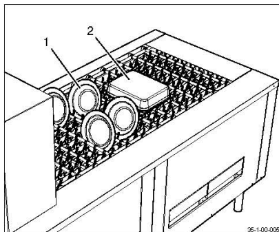
Infeed – placing items on the washing conveyor
